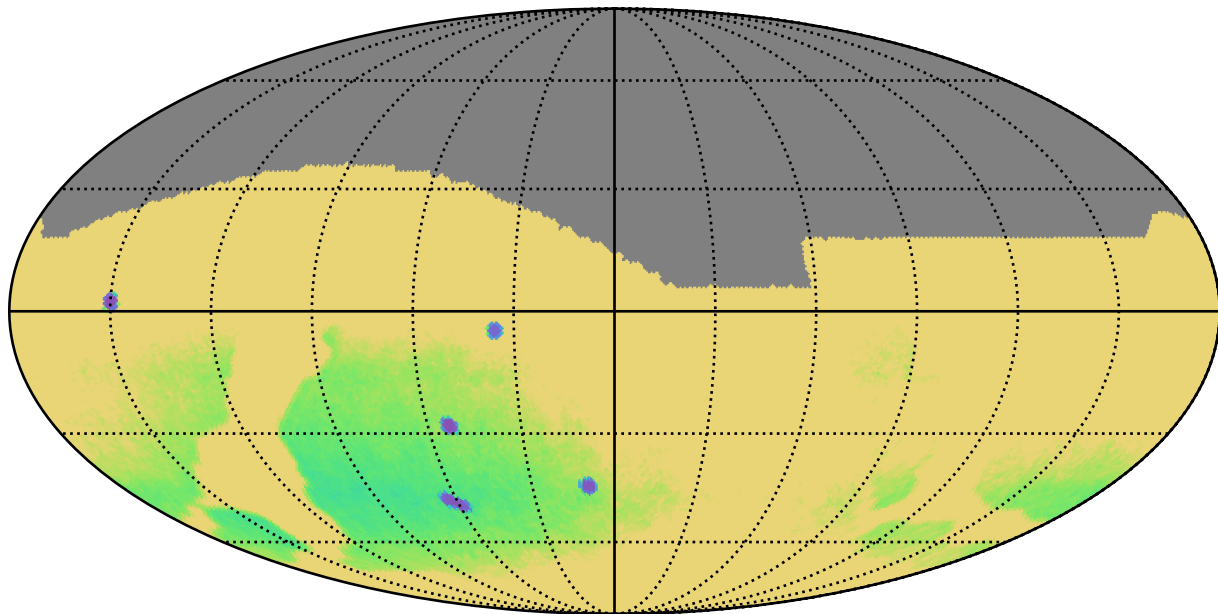
noroll_mjdp270_v3.4_10yrs : Parallax Uncert @ 22.4
