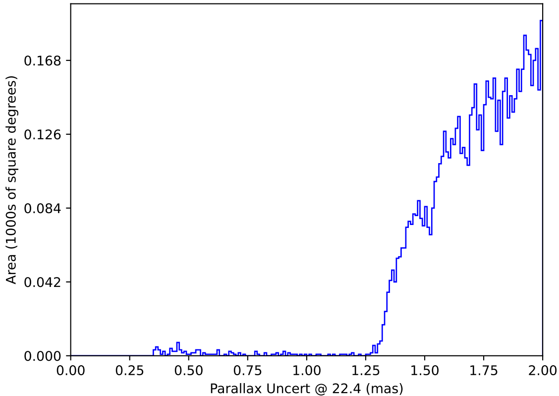
noroll_mjdp270_v3.4_10yrs : Parallax Uncert @ 22.4
