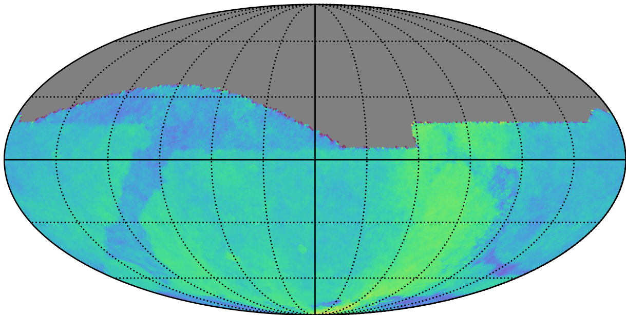
noroll_mjdp270_v3.4_10yrs : Parallax Coverage @ 24.0
