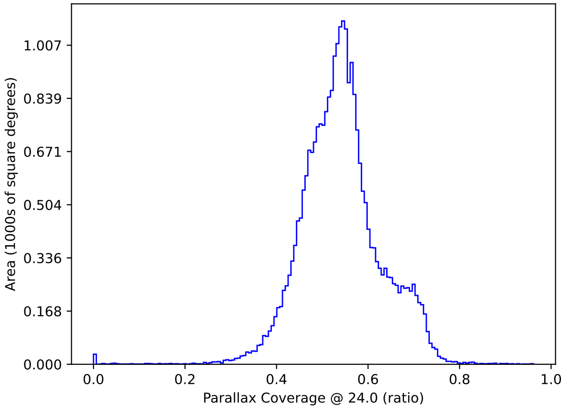
noroll_mjdp270_v3.4_10yrs : Parallax Coverage @ 24.0
