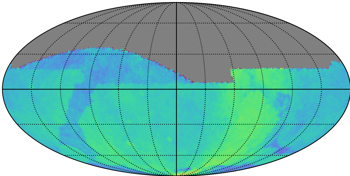
noroll_mjdp270_v3.4_10yrs : Parallax Coverage @ 22.4
