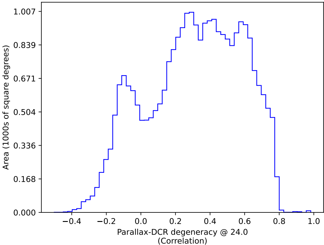
noroll_mjdp270_v3.4_10yrs : Parallax-DCR degeneracy @ 24.0
