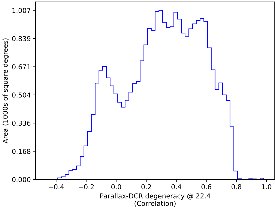
noroll_mjdp270_v3.4_10yrs : Parallax-DCR degeneracy @ 22.4
