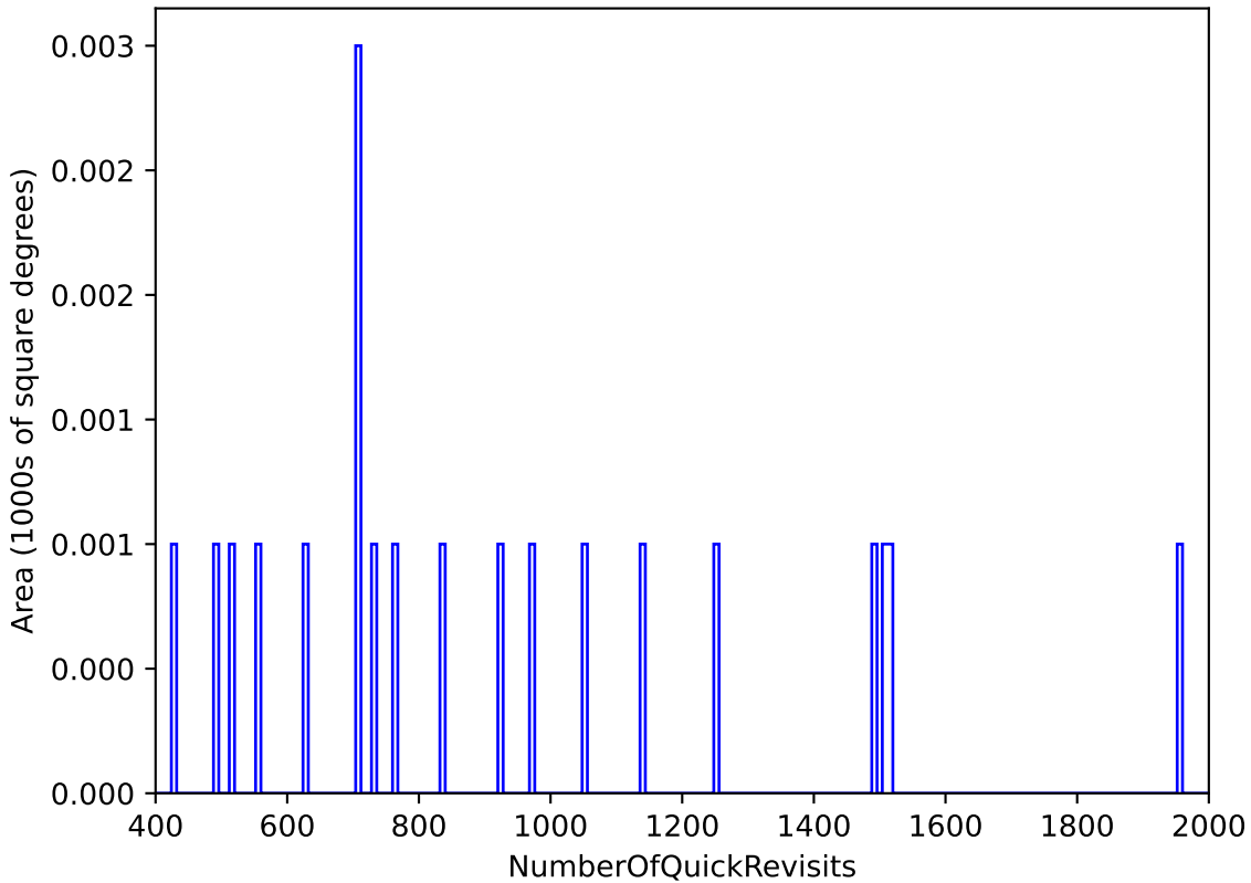
noroll_mjdp270_v3.4_10yrs : NumberOfQuickRevisits
