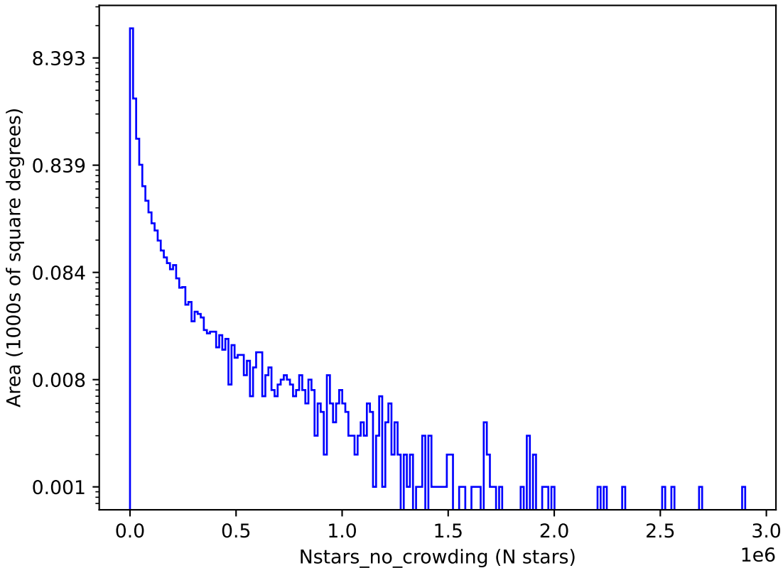
noroll_mjdp270_v3.4_10yrs u: Nstars_no_crowding
