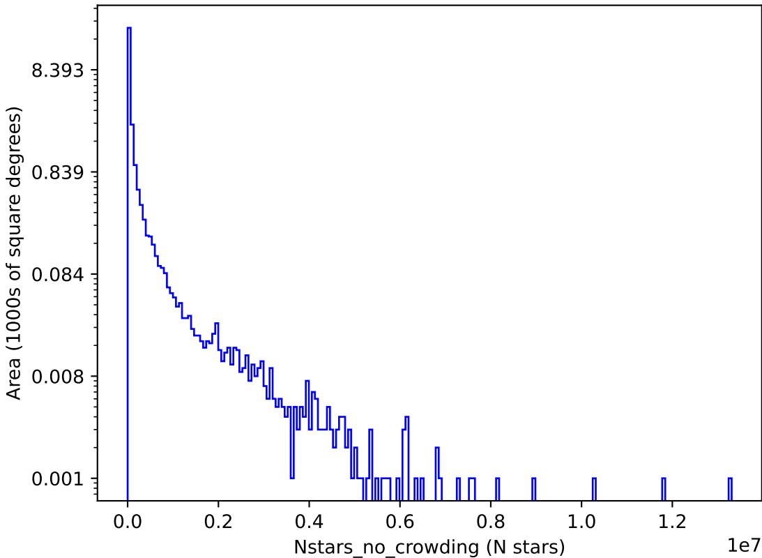
noroll_mjdp270_v3.4_10yrs g: Nstars_no_crowding
