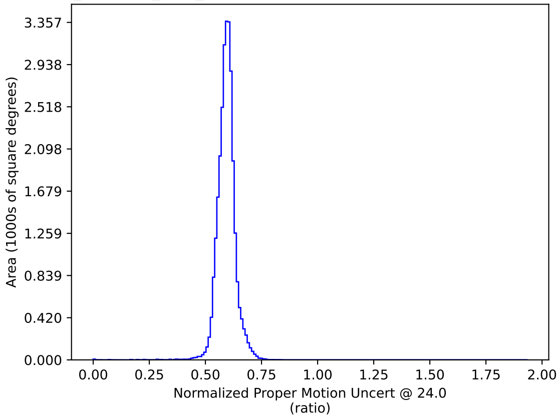
noroll_mjdp270_v3.4_10yrs : Normalized Proper Motion Uncert @ 24.0
