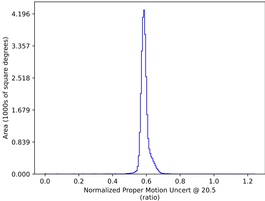
noroll_mjdp270_v3.4_10yrs : Normalized Proper Motion Uncert @ 20.5
