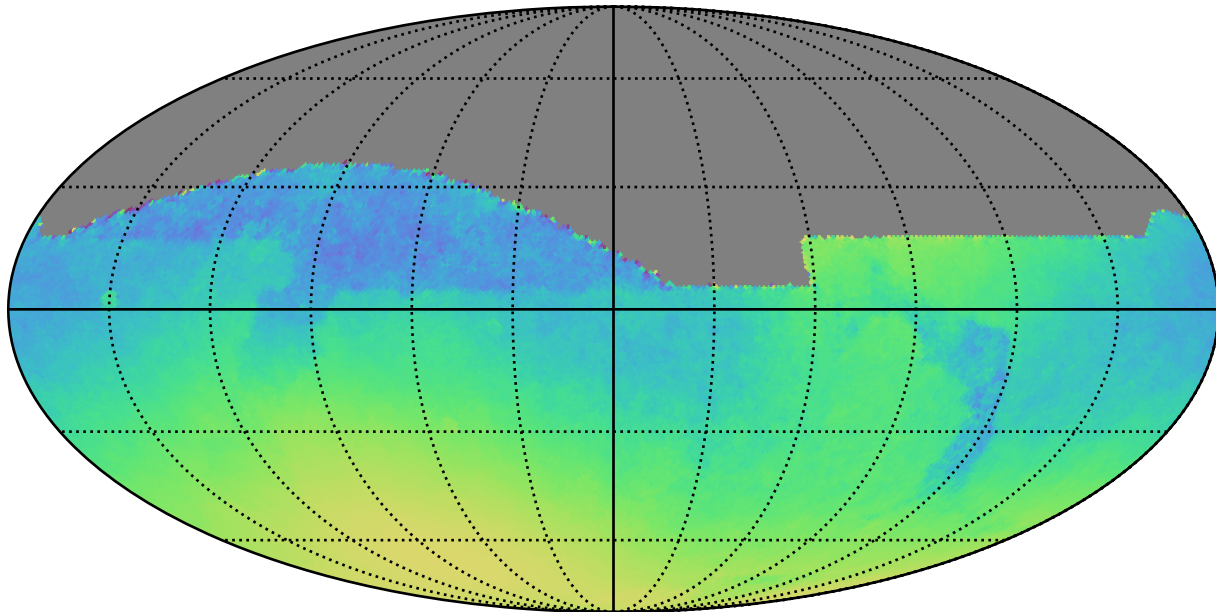
noroll_mjdp270_v3.4_10yrs : Normalized Parallax Uncert @ 24.0
