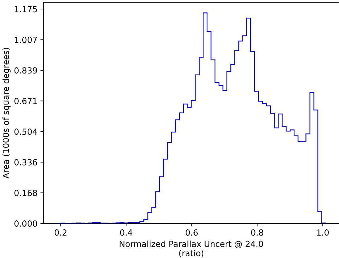
noroll_mjdp270_v3.4_10yrs : Normalized Parallax Uncert @ 24.0
