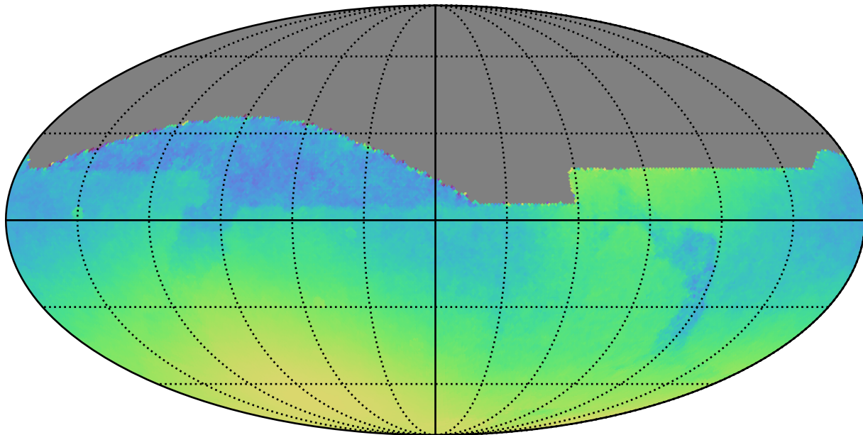
noroll_mjdp270_v3.4_10yrs : Normalized Parallax Uncert @ 22.4
