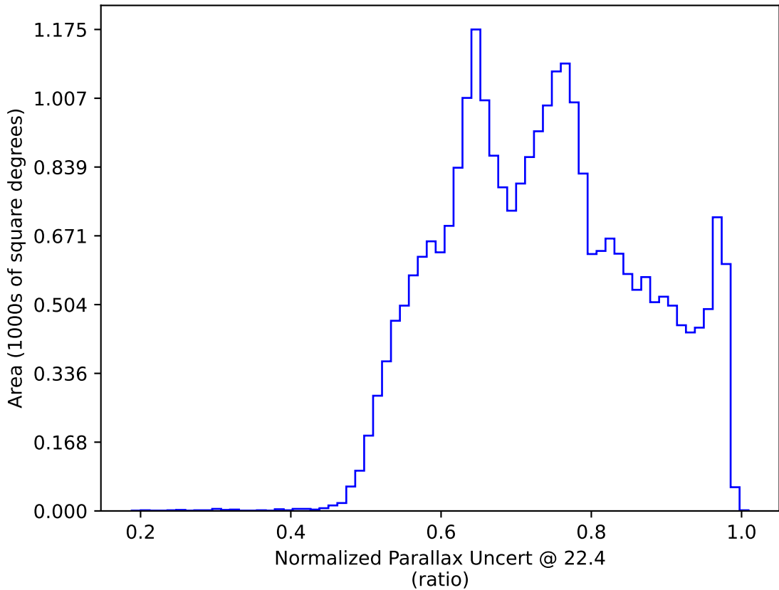
noroll_mjdp270_v3.4_10yrs : Normalized Parallax Uncert @ 22.4
