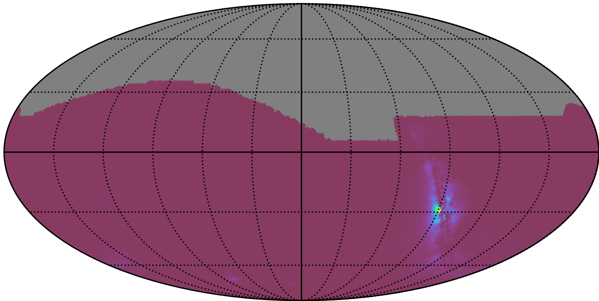
noroll_mjdp270_v3.4_10yrs : NlcPoints
