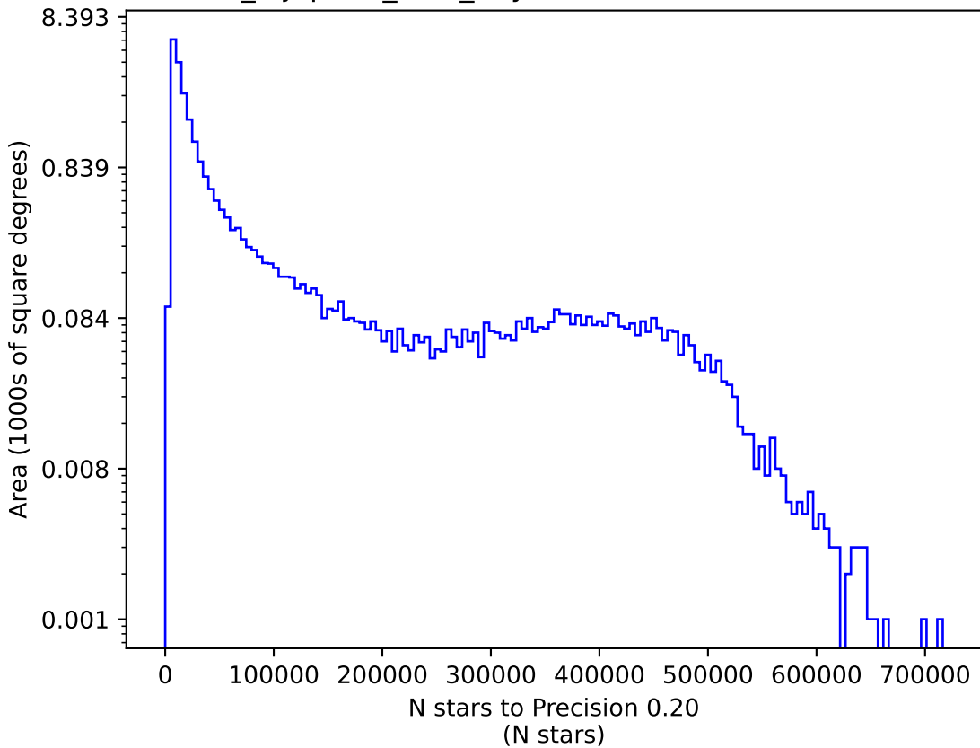
noroll_mjdp270_v3.4_10yrs z: N stars to Precision 0.20
