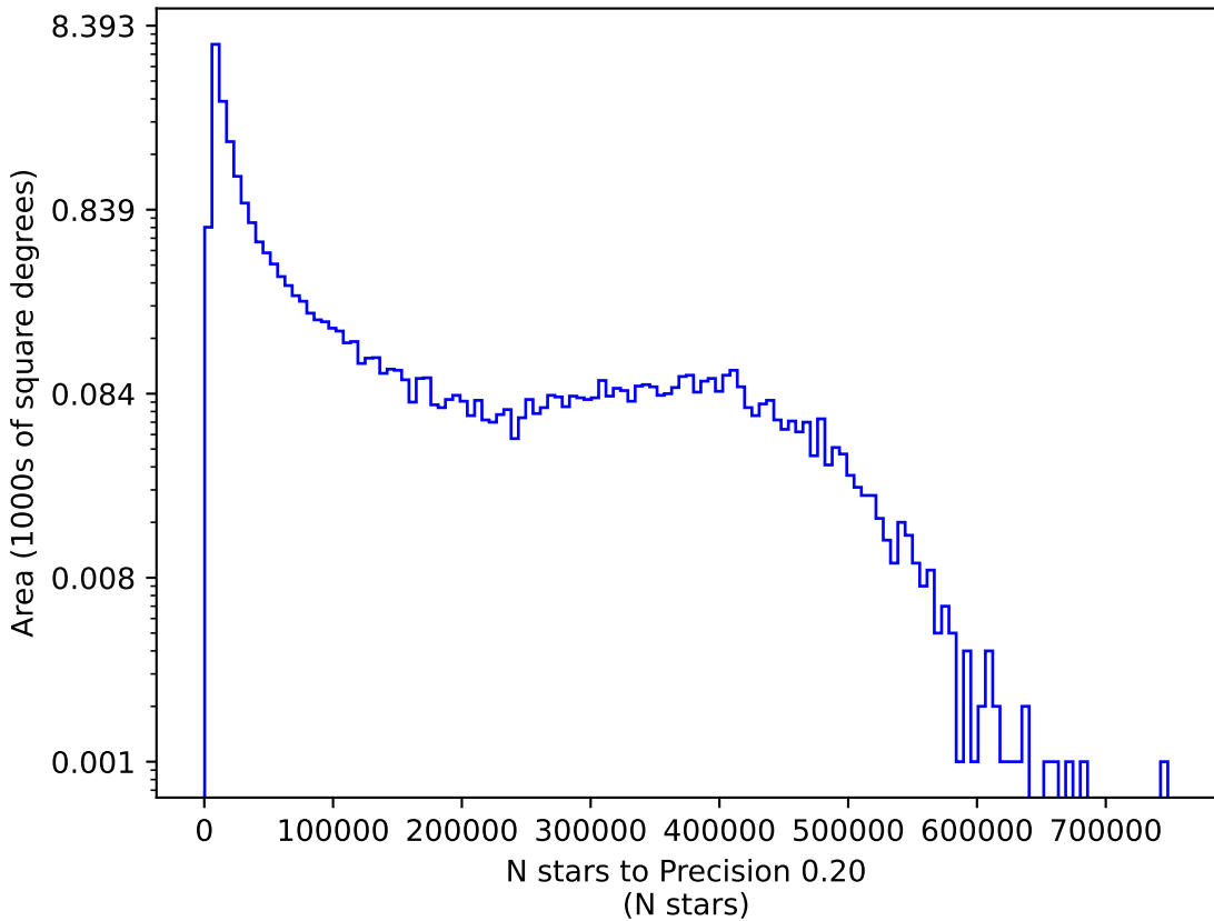
noroll_mjdp270_v3.4_10yrs y: N stars to Precision 0.20
