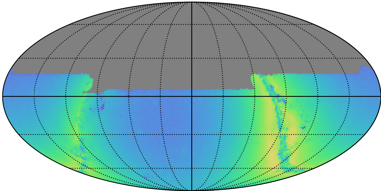
noroll_mjdp270_v3.4_10yrs u: N stars to Precision 0.20
