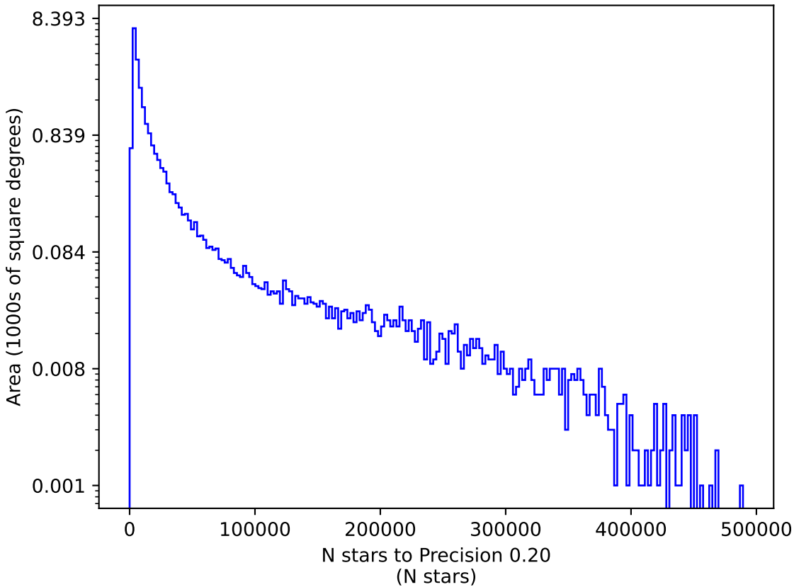
noroll_mjdp270_v3.4_10yrs u: N stars to Precision 0.20
