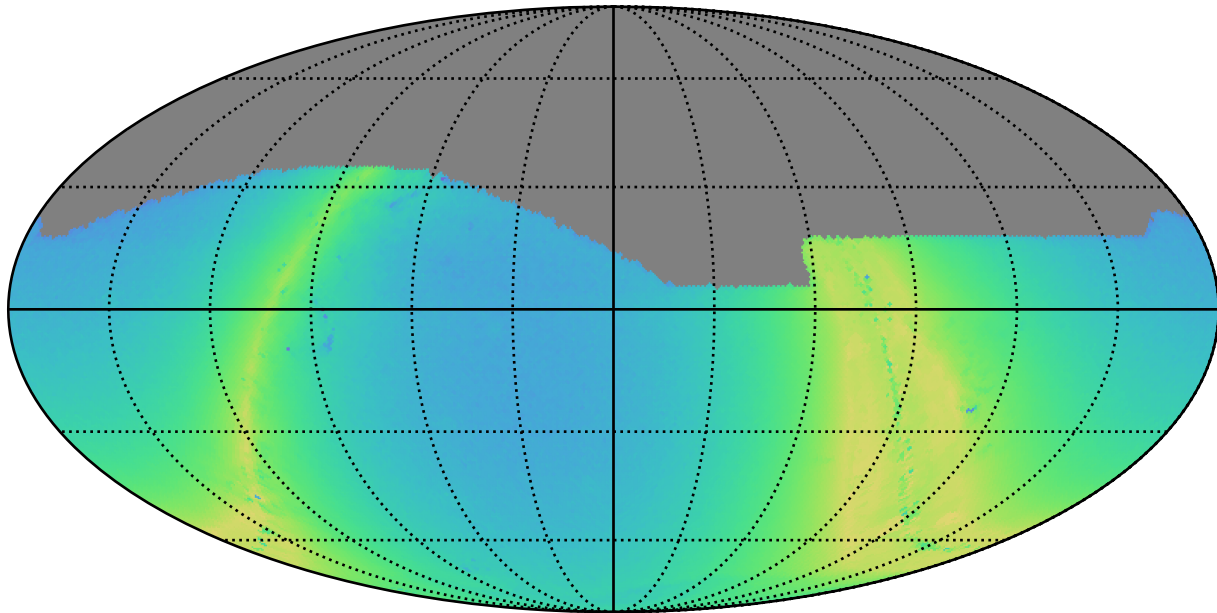
noroll_mjdp270_v3.4_10yrs r: N stars to Precision 0.20
