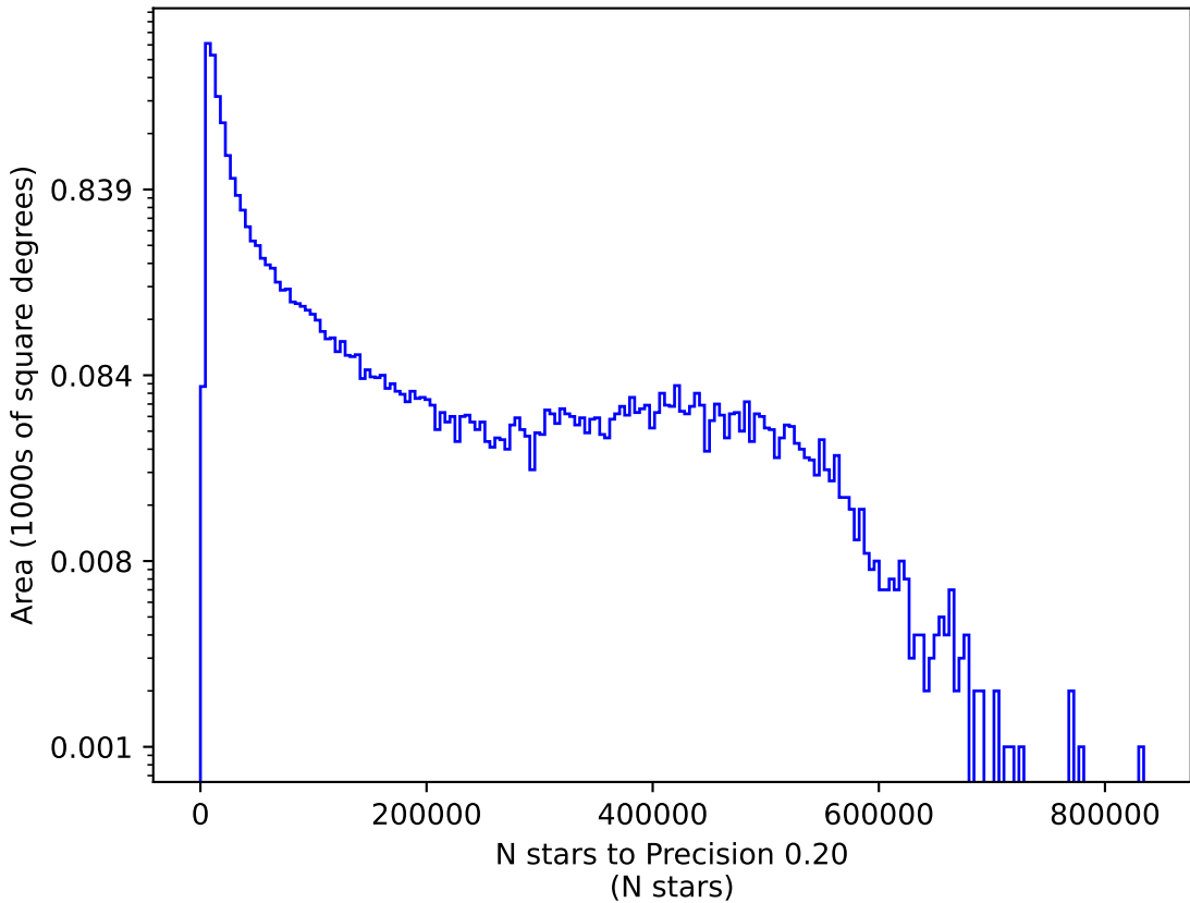
noroll_mjdp270_v3.4_10yrs r: N stars to Precision 0.20
