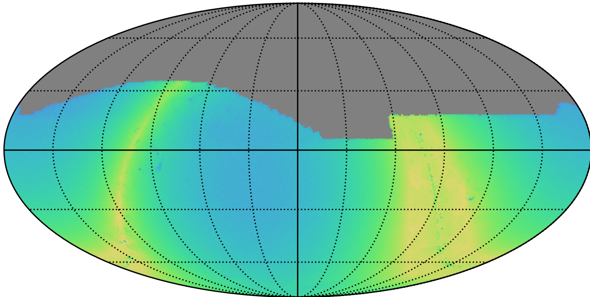
noroll_mjdp270_v3.4_10yrs i: N stars to Precision 0.20
