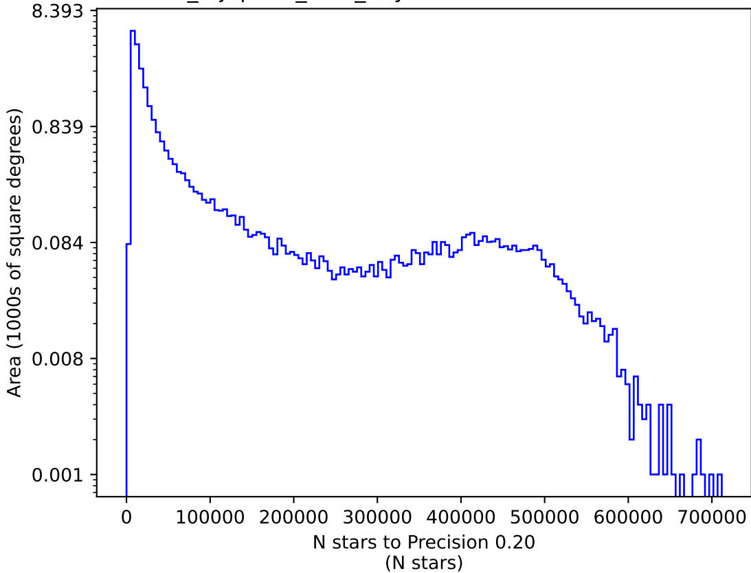
noroll_mjdp270_v3.4_10yrs i: N stars to Precision 0.20
