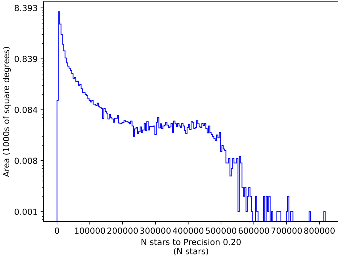
noroll_mjdp270_v3.4_10yrs g: N stars to Precision 0.20
