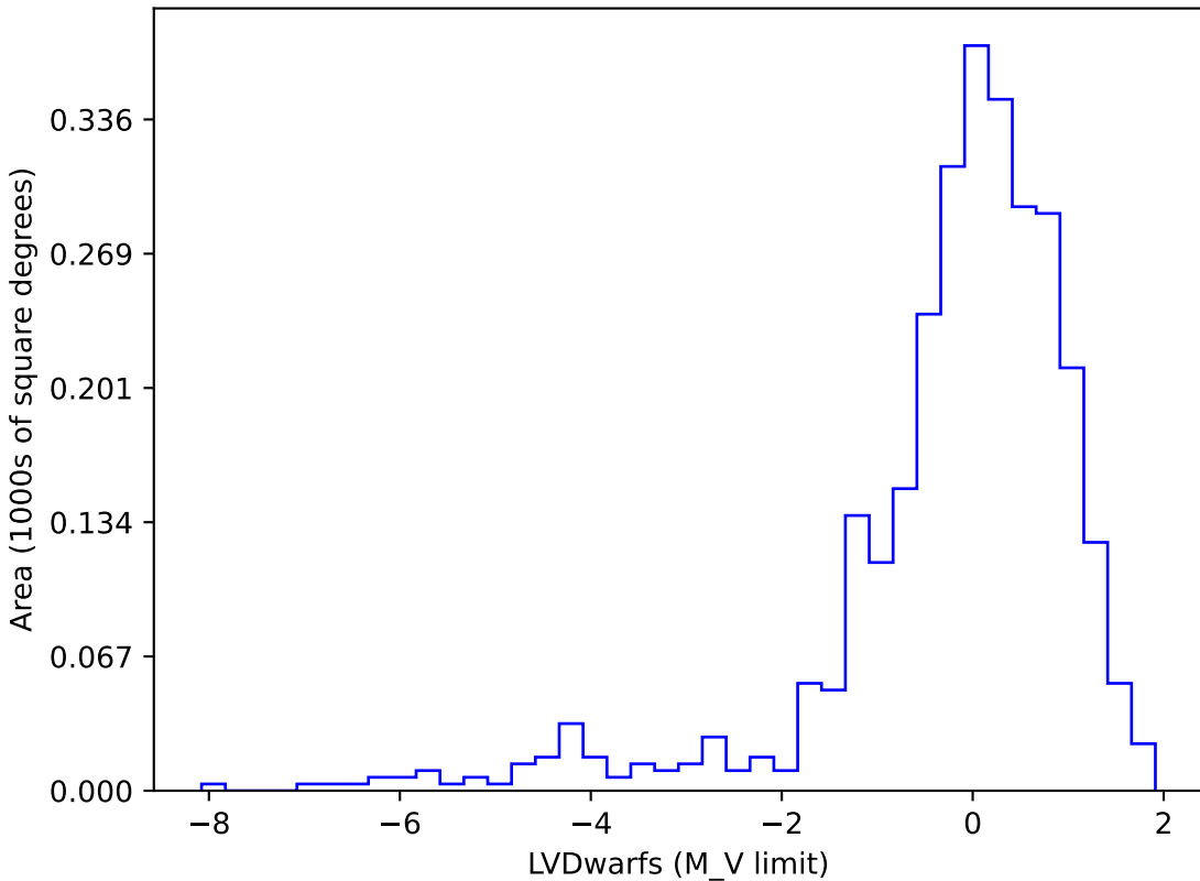
noroll_mjdp270_v3.4_10yrs gi SCP: LVDwarfs
