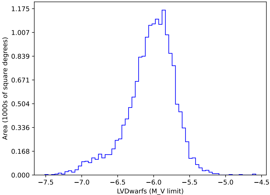
noroll_mjdp270_v3.4_10yrs gi: LVDwarfs
