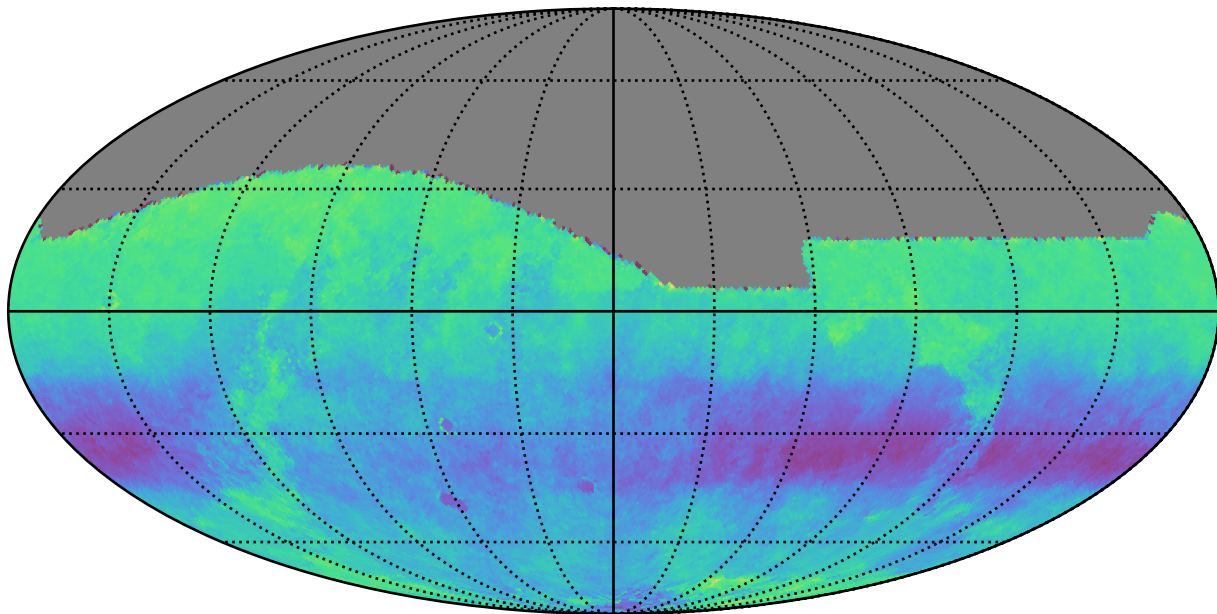
noroll_mjdp270_v3.4_10yrs r: Kuiper rotSkyPos
