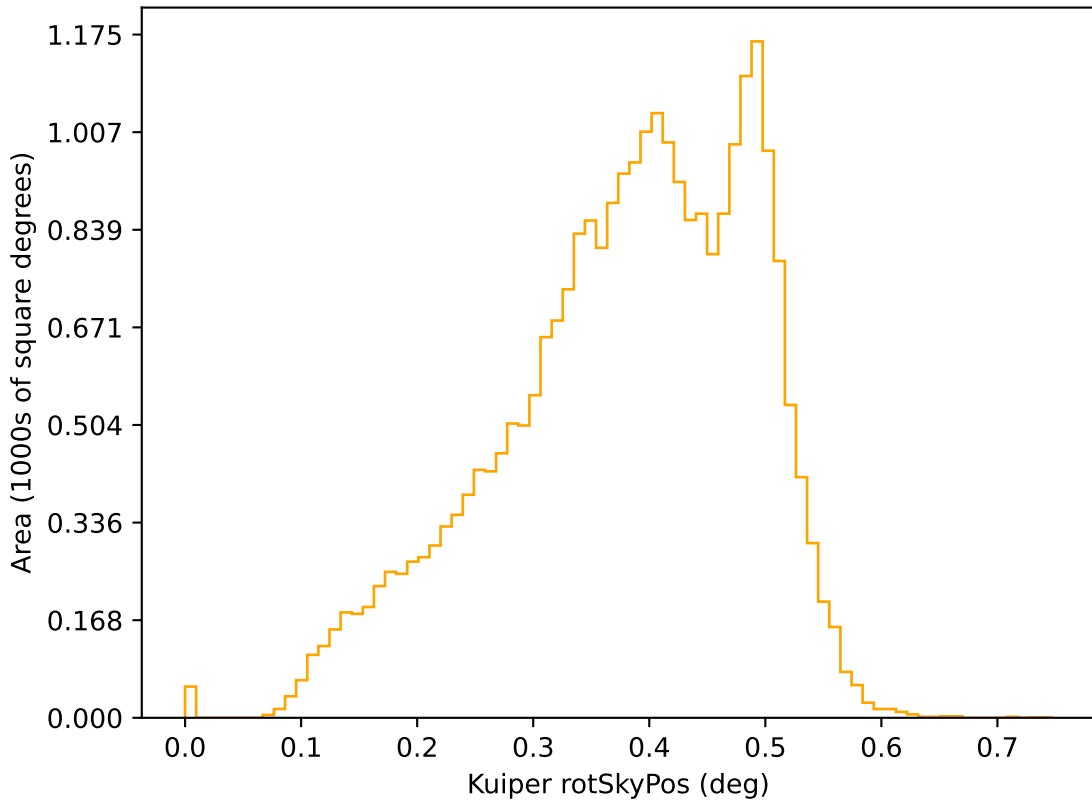
noroll_mjdp270_v3.4_10yrs r: Kuiper rotSkyPos
