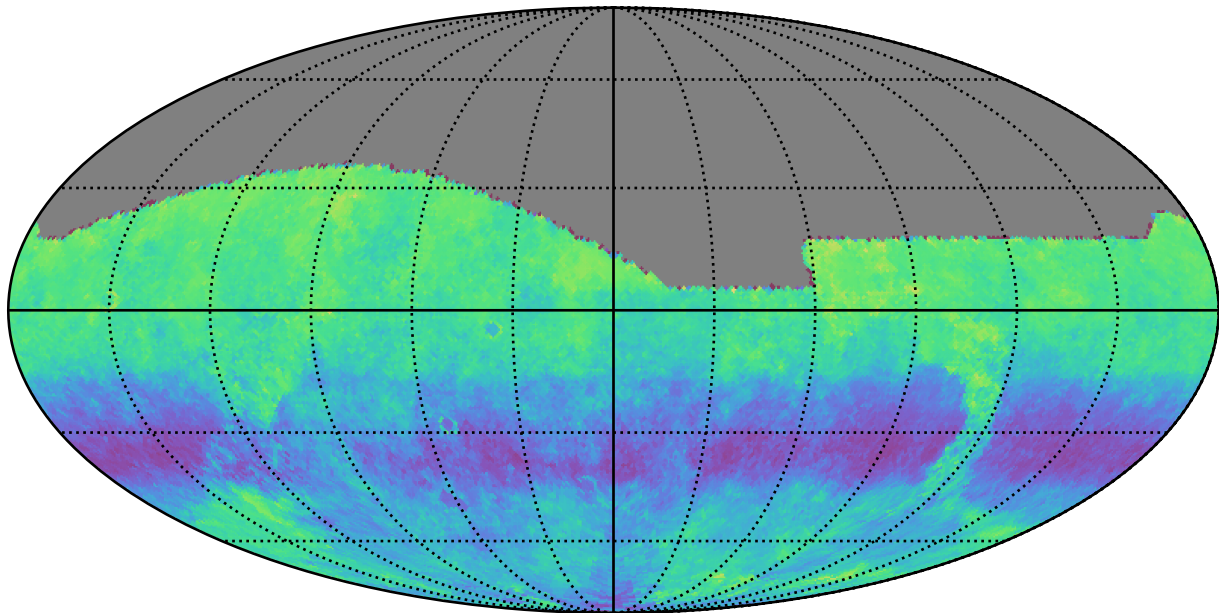
noroll_mjdp270_v3.4_10yrs g: Kuiper rotSkyPos
