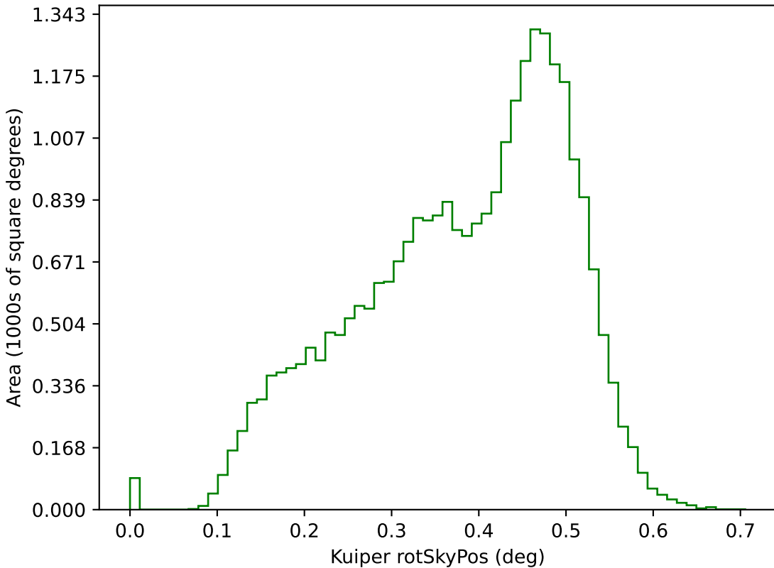
noroll_mjdp270_v3.4_10yrs g: Kuiper rotSkyPos
