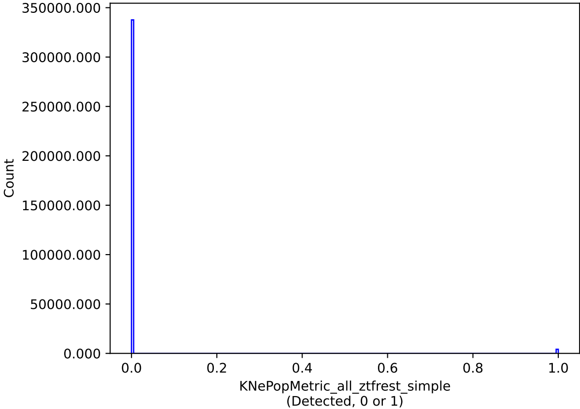
noroll_mjdp270_v3.4_10yrs all models: KNePopMetric_all_ztfrest_simple
