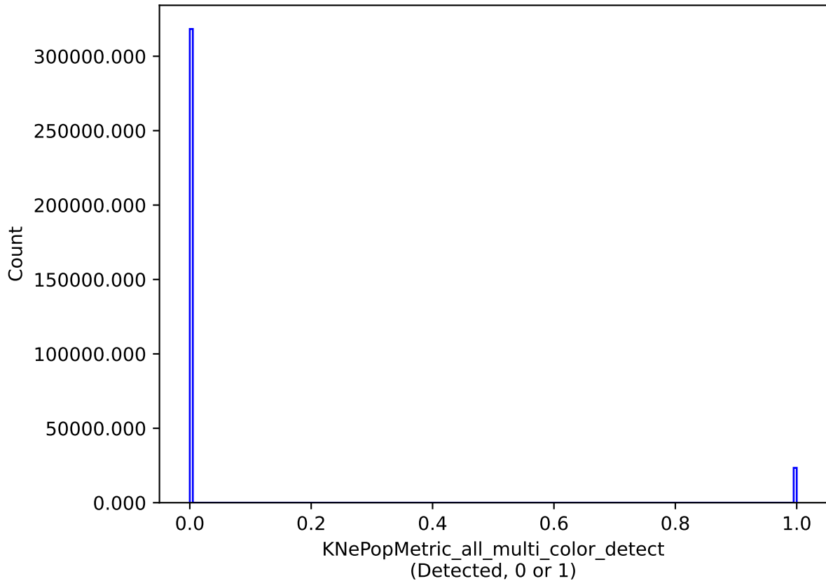
noroll_mjdp270_v3.4_10yrs all models: KNePopMetric_all_multi_color_detect
