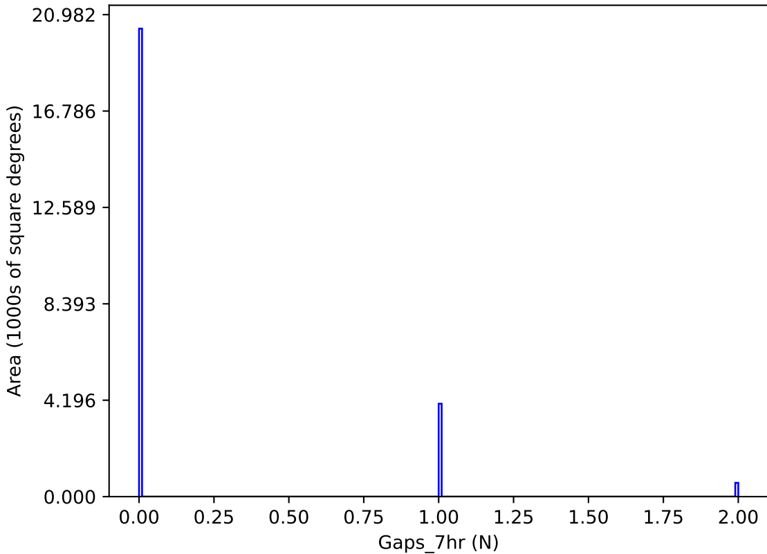
noroll_mjdp270_v3.4_10yrs y band: Gaps_7hr
