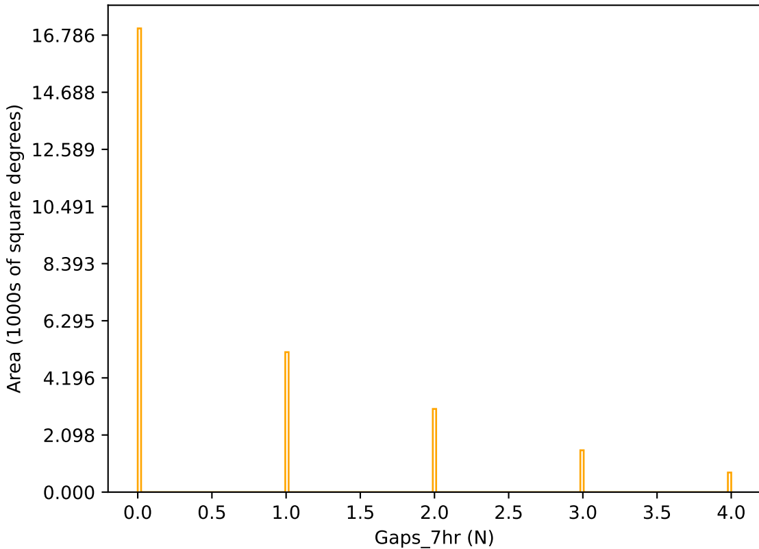
noroll_mjdp270_v3.4_10yrs r band: Gaps_7hr
