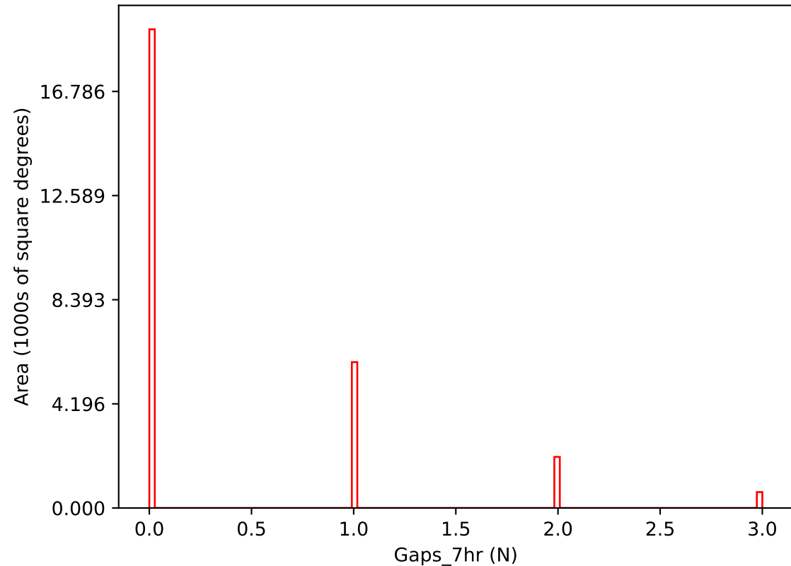
noroll_mjdp270_v3.4_10yrs i band: Gaps_7hr
