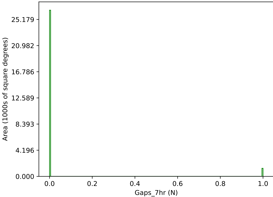
noroll_mjdp270_v3.4_10yrs g band: Gaps_7hr
