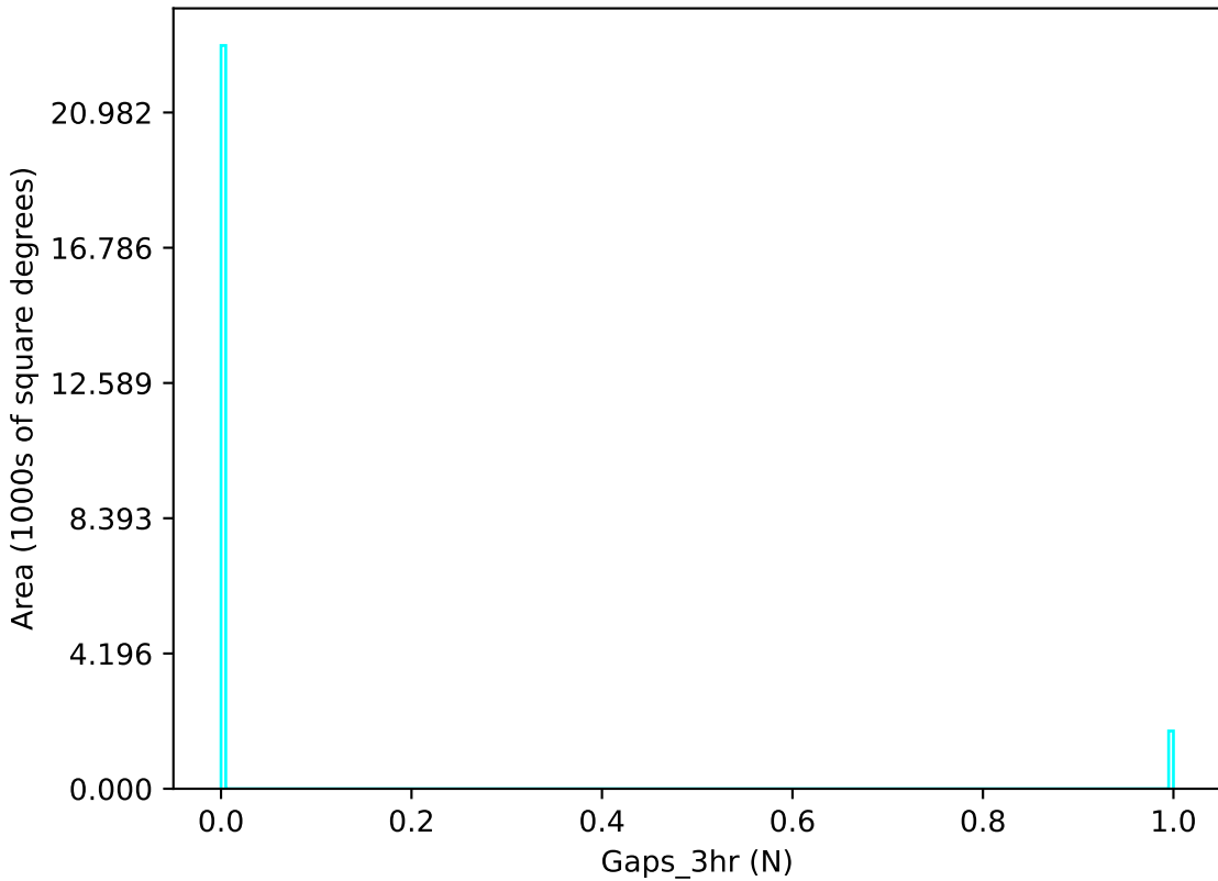
noroll_mjdp270_v3.4_10yrs u band: Gaps_3hr
