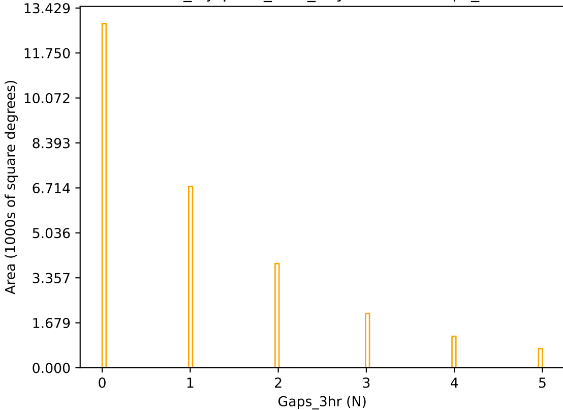
noroll_mjdp270_v3.4_10yrs r band: Gaps_3hr
