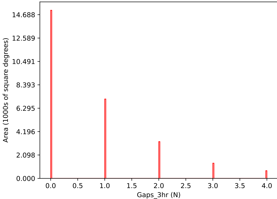
noroll_mjdp270_v3.4_10yrs i band: Gaps_3hr
