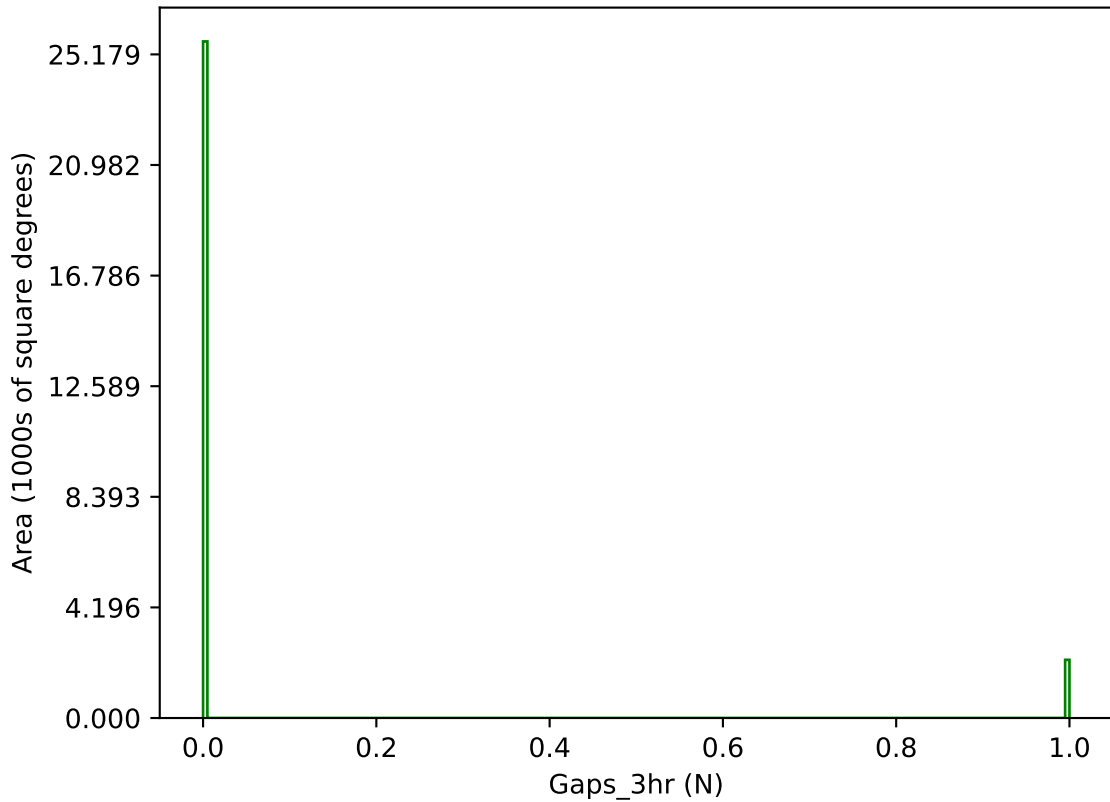
noroll_mjdp270_v3.4_10yrs g band: Gaps_3hr
