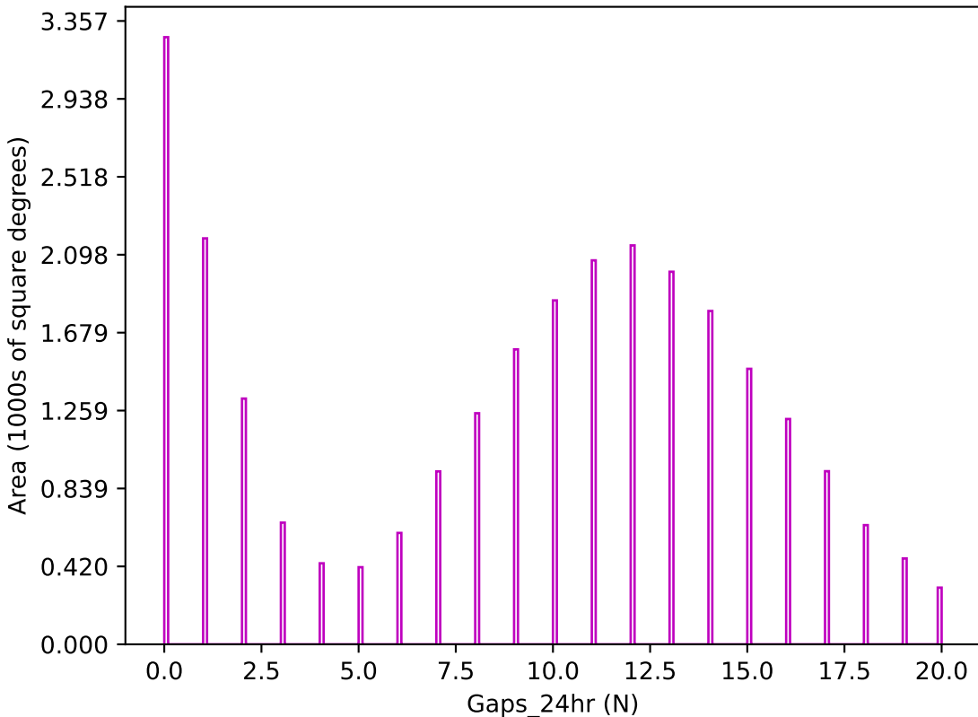
noroll_mjdp270_v3.4_10yrs z band: Gaps_24hr
