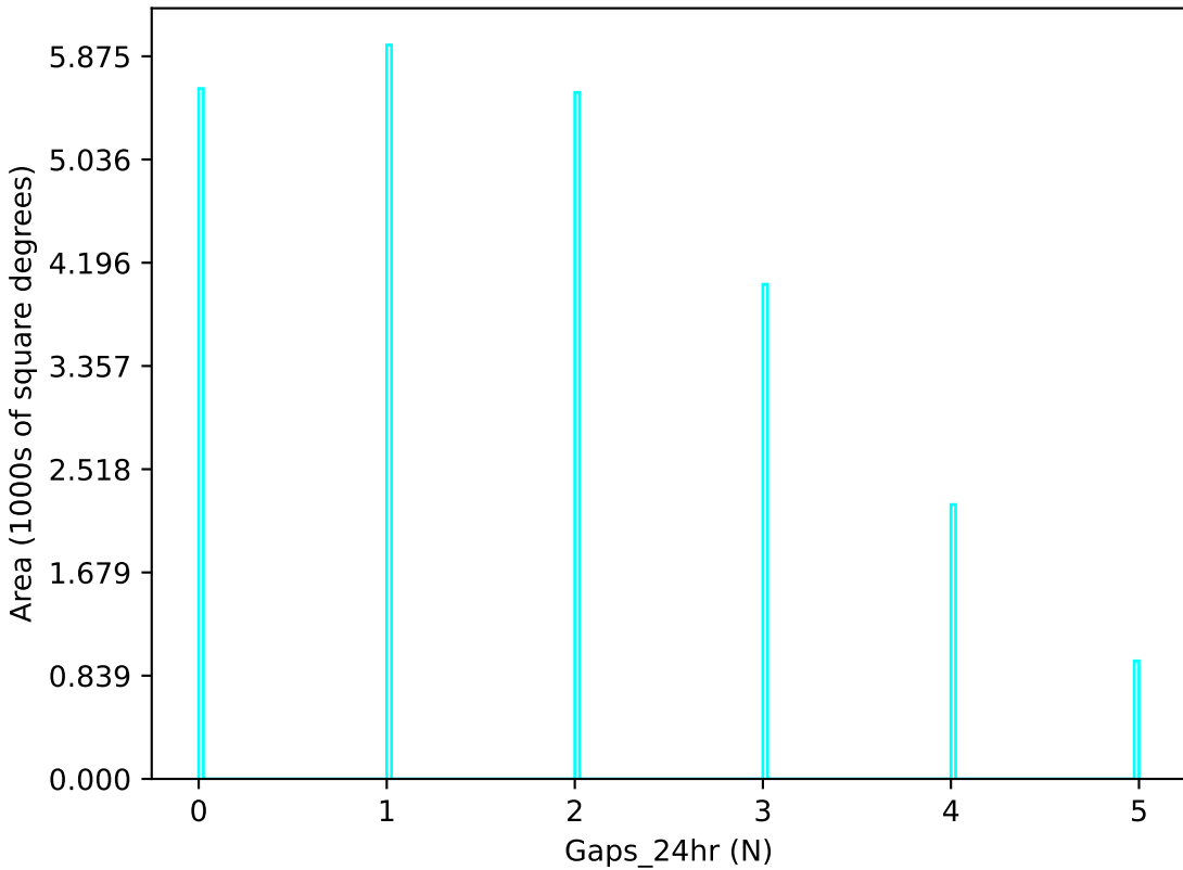
noroll_mjdp270_v3.4_10yrs u band: Gaps_24hr
