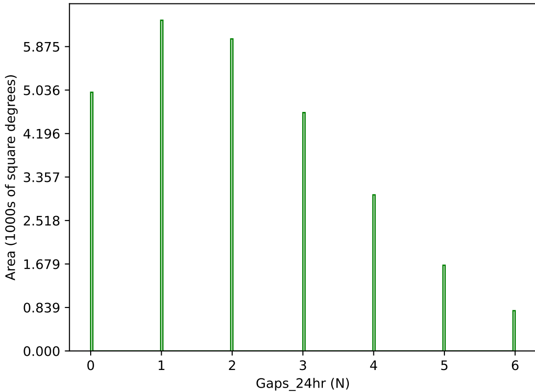
noroll_mjdp270_v3.4_10yrs g band: Gaps_24hr
