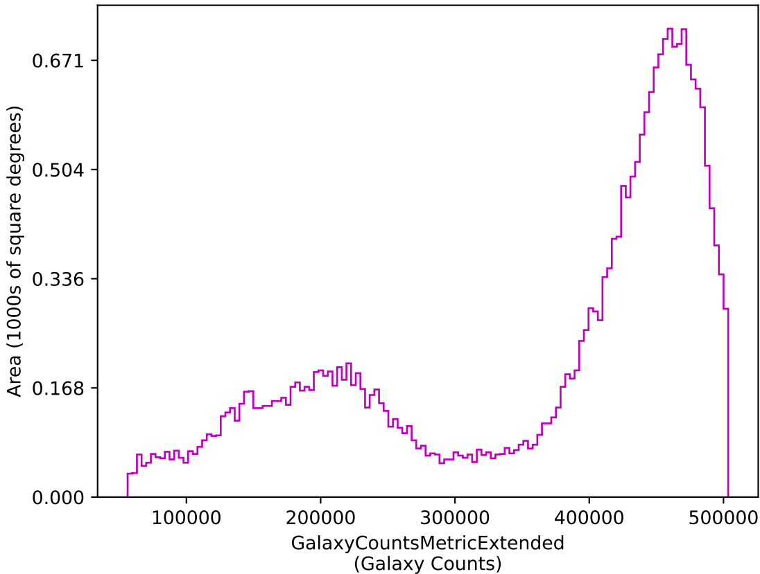
noroll_mjdp270_v3.4_10yrs z: GalaxyCountsMetricExtended
