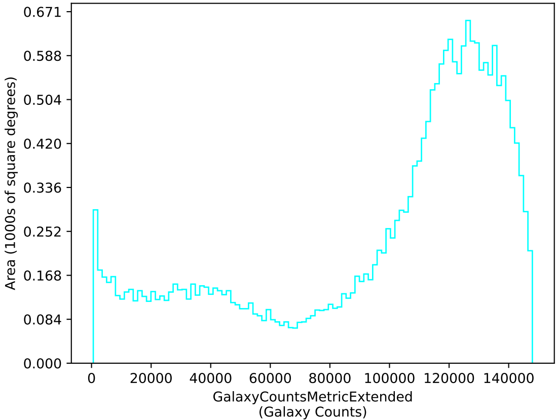
noroll_mjdp270_v3.4_10yrs u: GalaxyCountsMetricExtended
