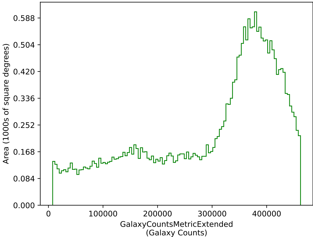
noroll_mjdp270_v3.4_10yrs g: GalaxyCountsMetricExtended
