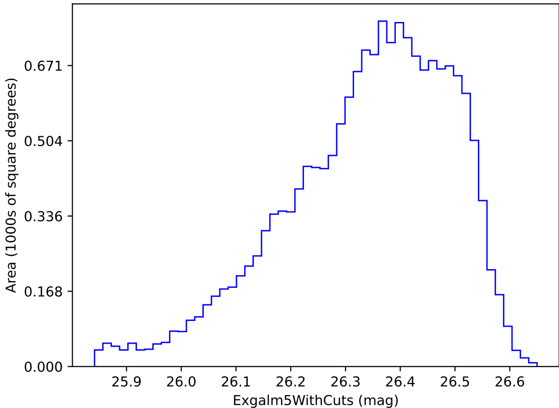
noroll_mjdp270_v3.4_10yrs i band non-DD year 9: ExgalM5WithCuts
