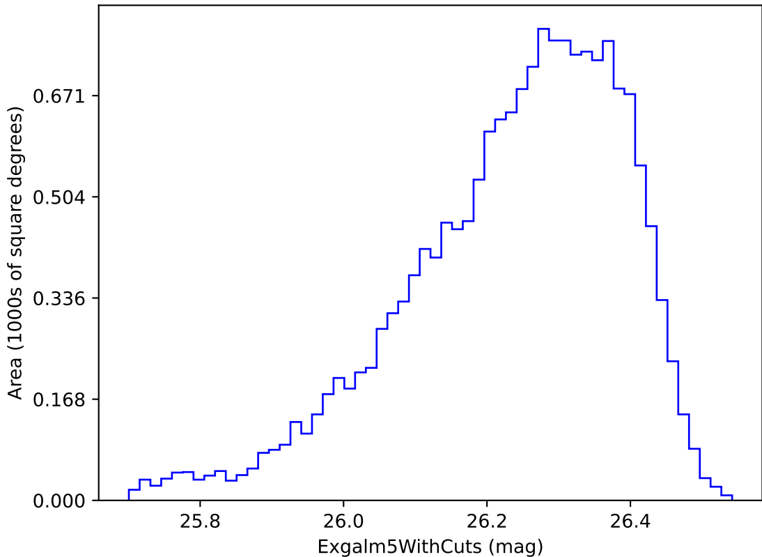
noroll_mjdp270_v3.4_10yrs i band non-DD year 7: ExgalM5WithCuts
